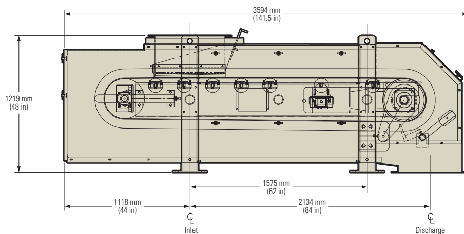
SIDE VIEW
