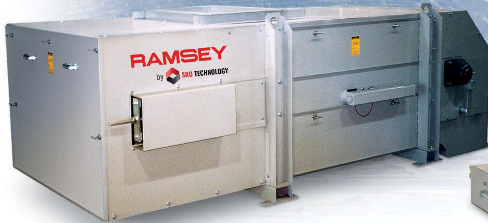
Ramsey Model 90-100 Heavy Duty Weighbelt Feeder
