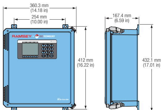
Field Mount Model
