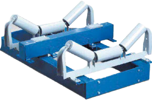
Ramsey Series 14 belt scale A top-of-the-range scale that sets the global standard for accuracy and performance for loadout, inventory monitoring and basis-of-payment applications. Accuracy +/-0.125%
