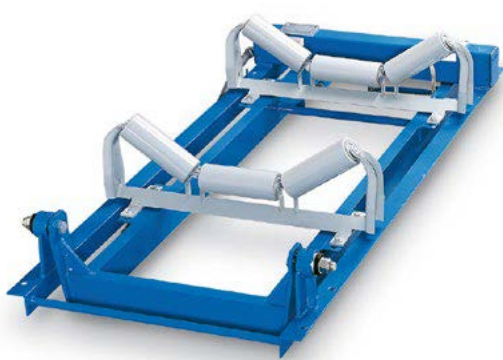
Ramsey Series 17 belt scale A multi-idler scale for plants and processes that run at high speed or require high accuracy. Accuracy +/-0.25%
